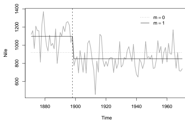
Figure 5: Fitted models for the Nile data
