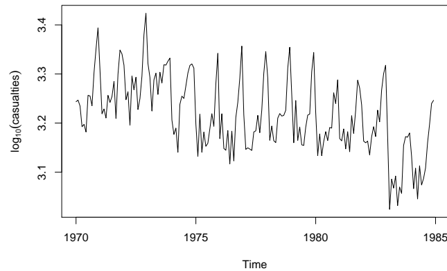
Figure 6: The seatbelt data
