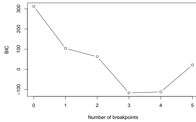
Figure 11: BIC for models with m breakpoints
