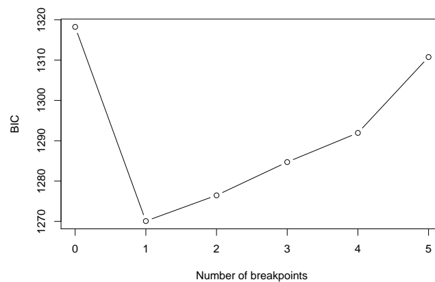
Figure 4: BIC for models with m breakpoints
