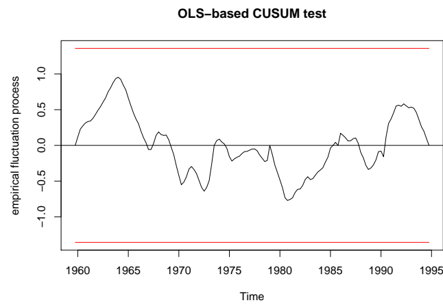
Figure 12: OLS-based CUSUM process for the oil price data
