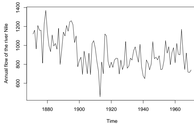
Figure 1: The Nile data
