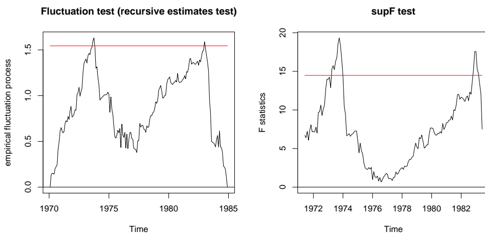
Figure 7: Structural change tests for the seatbelt data
