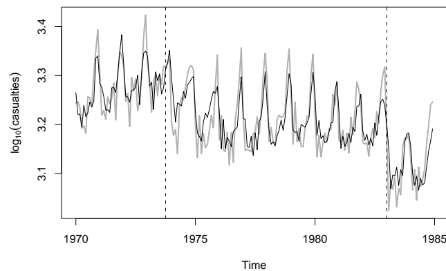
Figure 9: Fitted model for the seatbelt data
