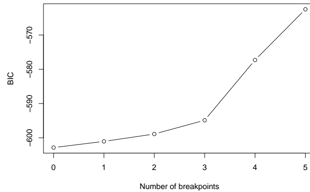
Figure 8: BIC for models with m breakpoints
