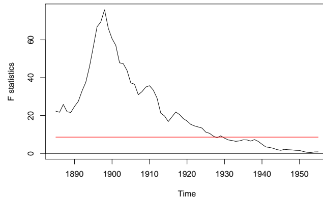
Figure 3: F statistics for the Nile data
