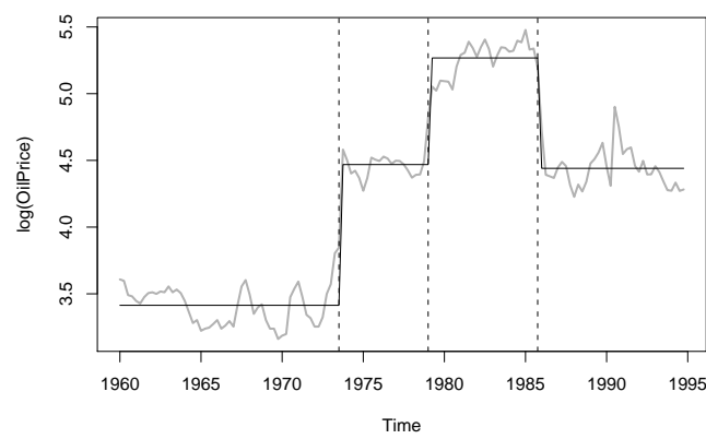
Figure 13: Fitted model for the oil price data
