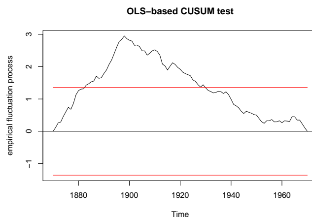
Figure 2: OLS-based CUSUM process for the Nile data
